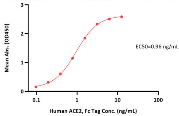
Biotinylated SARS-CoV-2 Spike RBD (Y449H, E484K, N501Y), His,Avitag ELISA 0.5 µg of Biotinylated SARS-CoV-2 Spike RBD (Y449H, E484K, N501Y), His,Avitag per well
