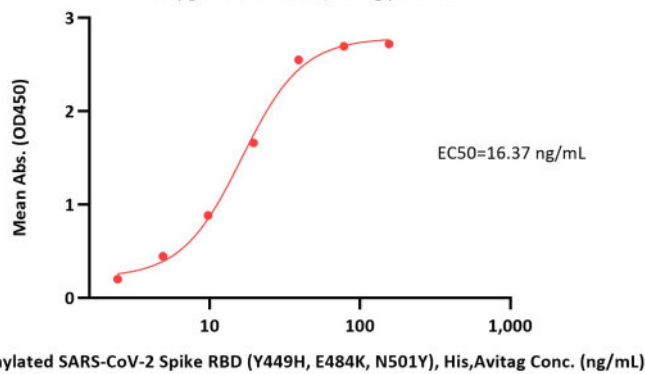
Biotinylated SARS-CoV-2 Spike RBD (Y449H, E484K, N501Y), His,Avitag ELISA 0.5 µg of Human ACE2, Fc Tag per well
