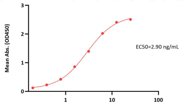
Biotinylated SARS-CoV-2 Spike RBD (Y449H, E484K, N501Y), His,Avitag ELISA 0.5 µg of Biotinylated SARS-CoV-2 Spike RBD (Y449H, E484K, N501Y), His,Avitag per well
