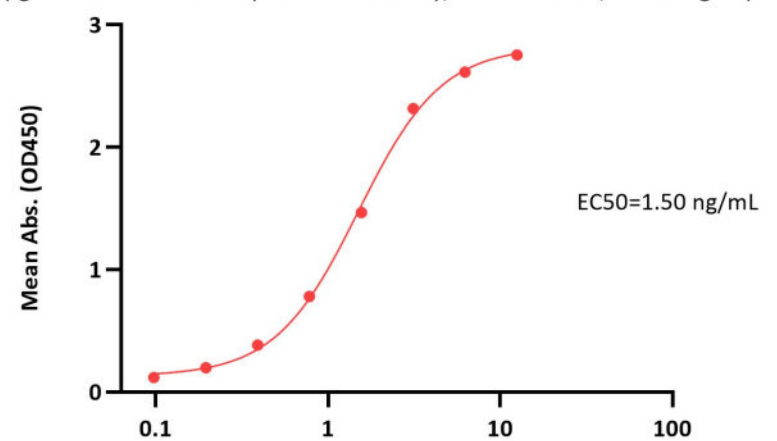
Biotinylated SARS-CoV-2 Spike RBD (Y449H, E484K, N501Y), His,Avitag ELISA 0.1 µg of Anti-SARS-CoV-2 Spike RBD Antibody, Chimeric mAb, Human IgG1 per well
