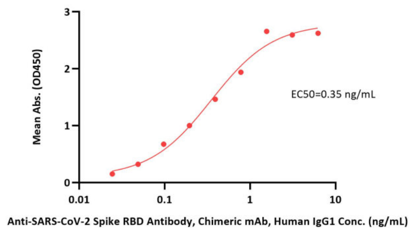
SARS-CoV-2 Spike RBD (L452R, T478K, N501Y), His Tag ELISA 0.1 µg of SARS-CoV-2 Spike RBD (L452R, T478K, N501Y), His Tag per well
